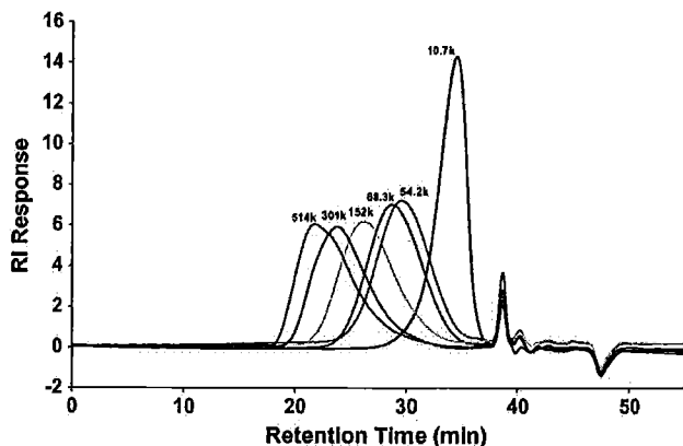
Fig. 1. Overlay of chromatograms of the six broad calibration standards (Mw labelled).
